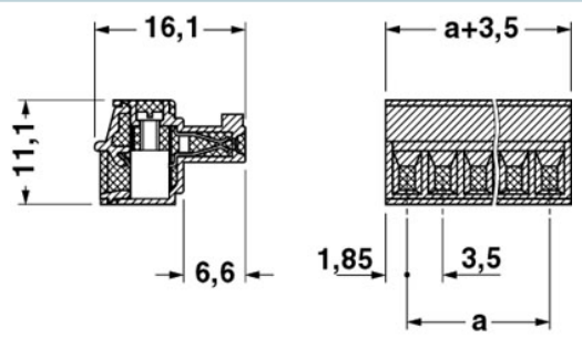
Dimensioned drawing
